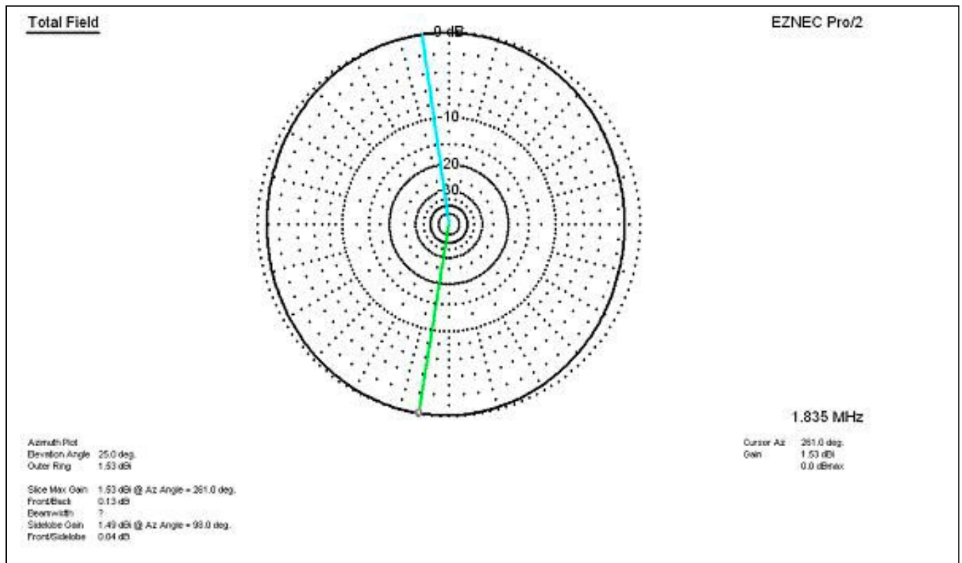
Fig. 5 - Azimuth Plot of Inverted U
