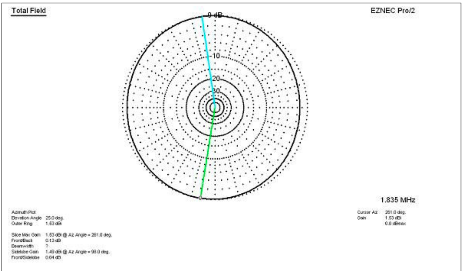
Figure 3 – Elevation Plot – Take Off Angle is 26 Degrees
