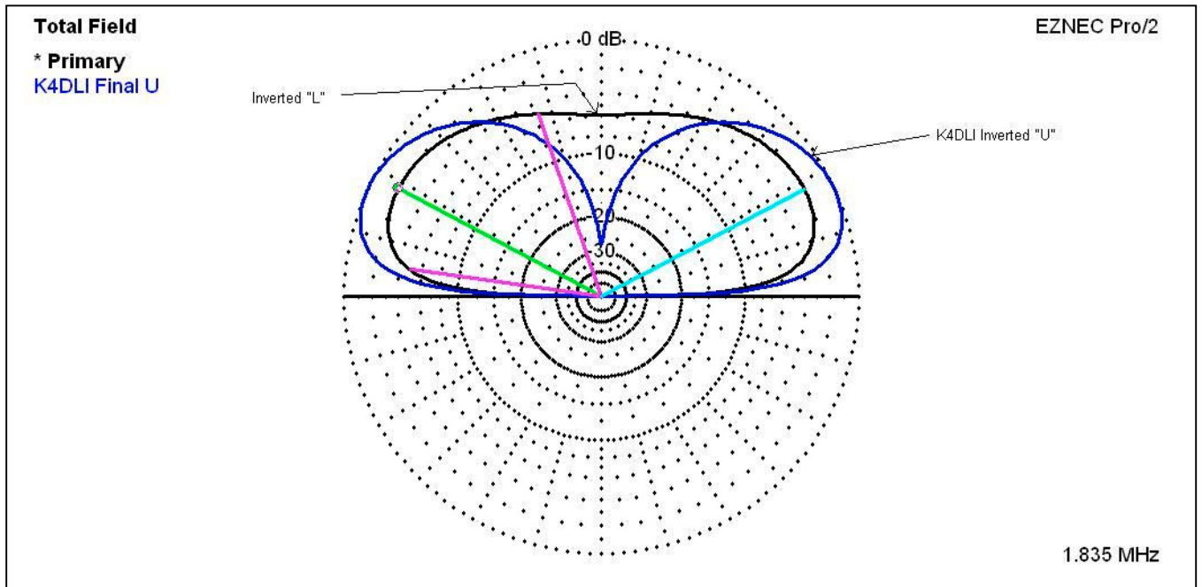
Fig. 4 - Comparison plot of the Inverted "L" and the Inverted "U" Antenna
